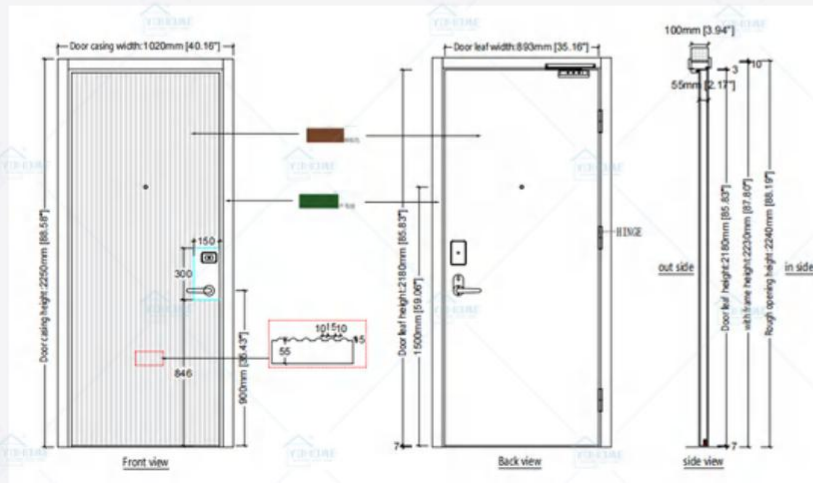
European Standard 30-minute Fire Door
