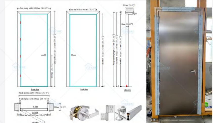
Stainless Steel Door
