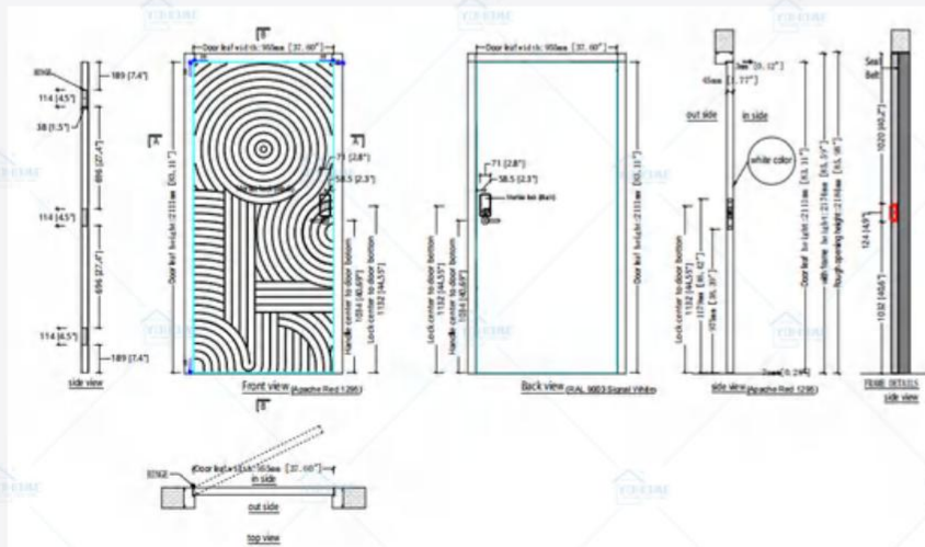
UL 20min Wooden Fire Door
