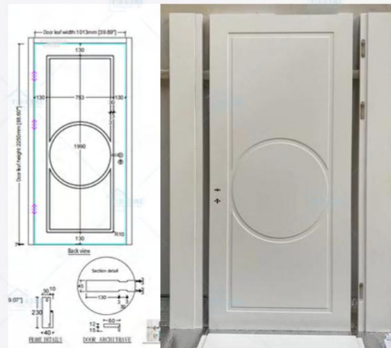
Gym&Spa Room Door
