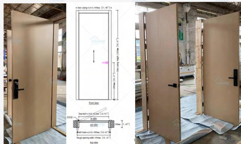
Bedroom/Bathroom Door
