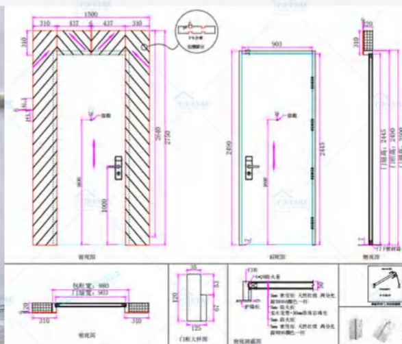
Entrance Door (Left Hand Inswing)
