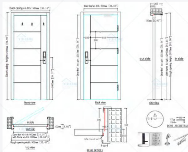
Wooden Fire-rated Door
