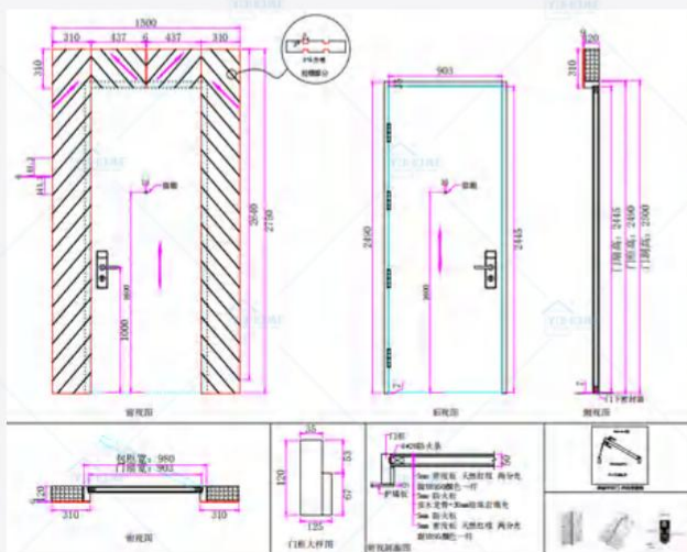
Entrance Door (Right Hand Inswing)
