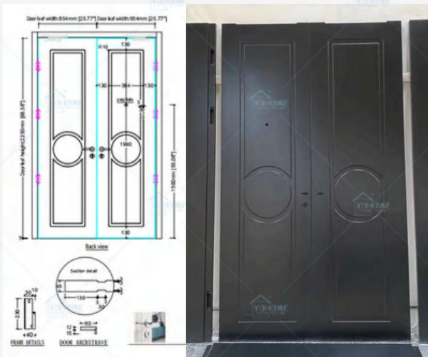
Hotel Room Door
