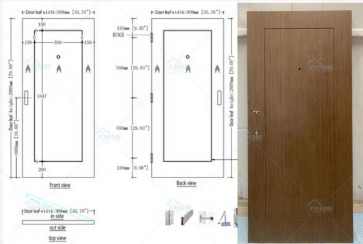
UL Fire-rated Door
