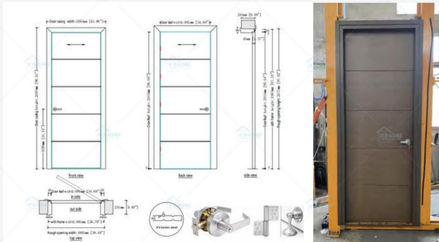
Steel-Wood Composite Door
