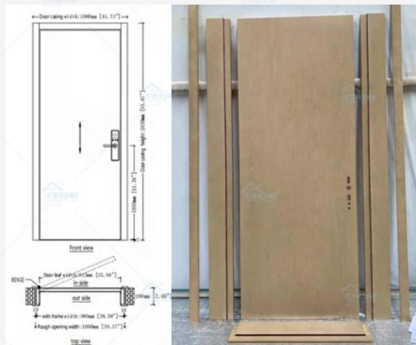
Main Access Door
