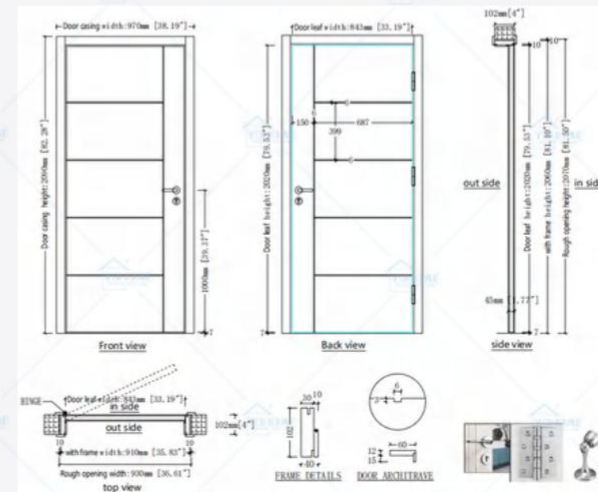
Composite Wooden Door
