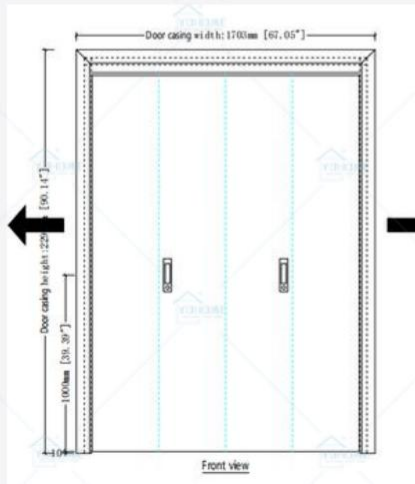
Double Folding Door
