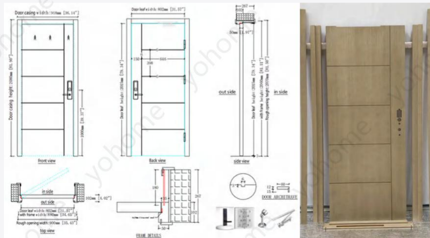
Wooden Fire-rated Door
