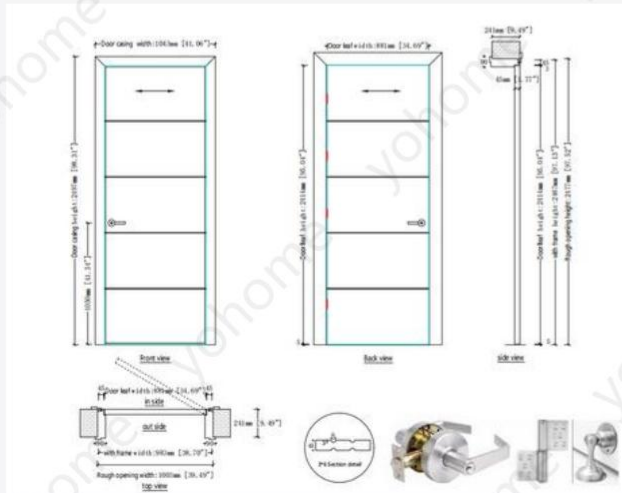
Steel-Wood Composite Door
