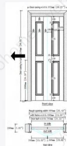
Kitchen Pantry Door
