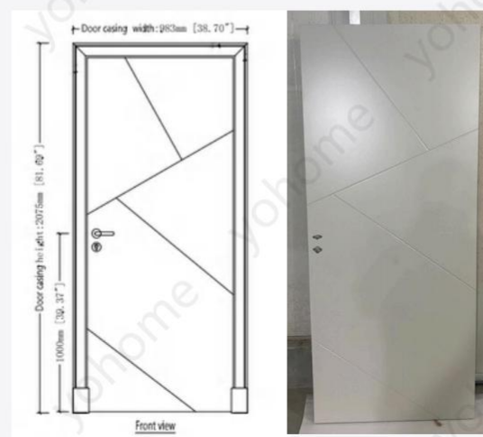
Interior Wooden Door
