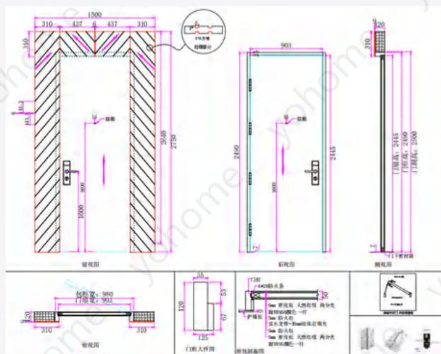
Entrance Door (Right Hand Inswing)
