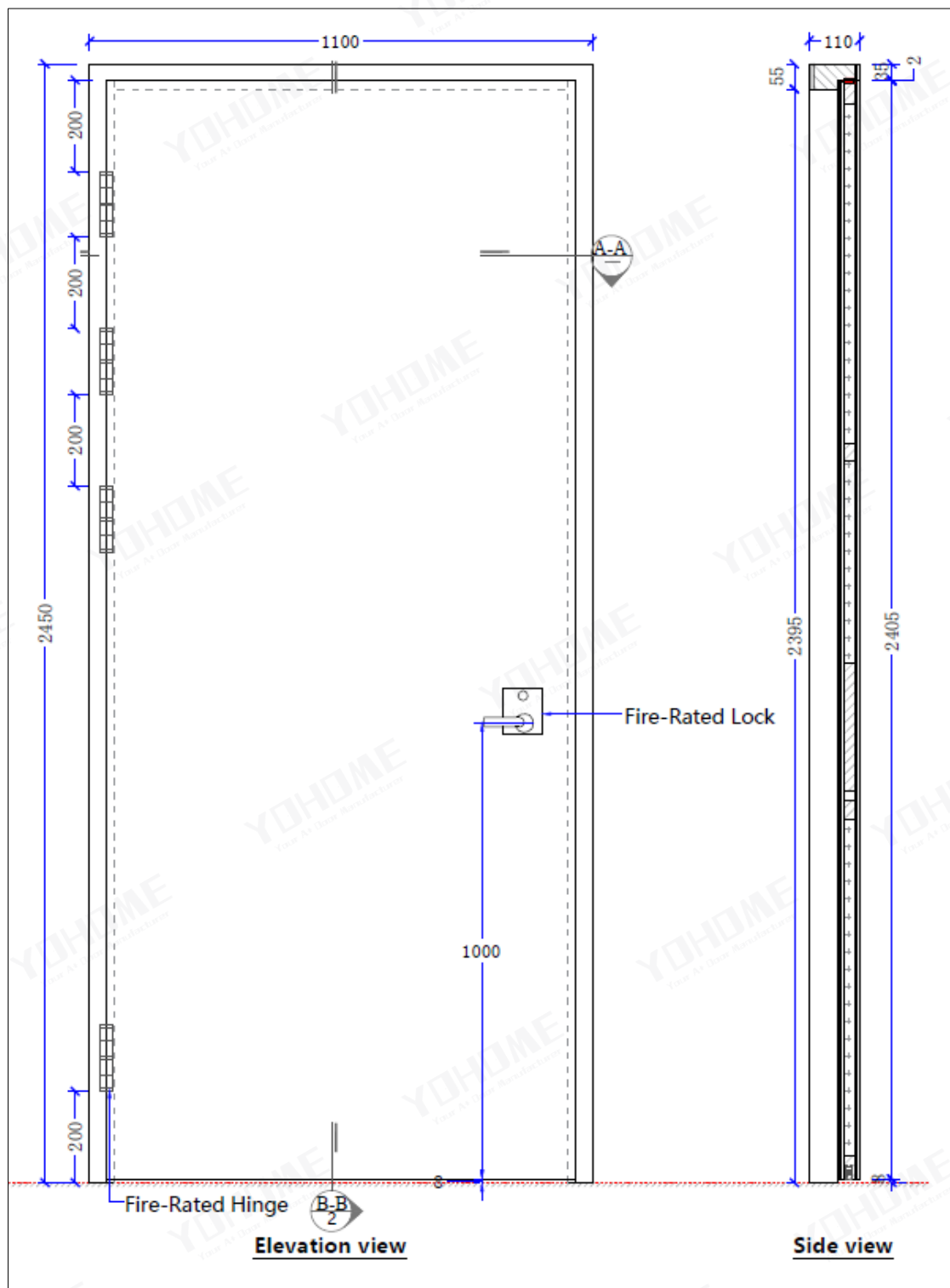
Drawing of UL 20mins single leaf wooden fire door and frame, Model YH-01
