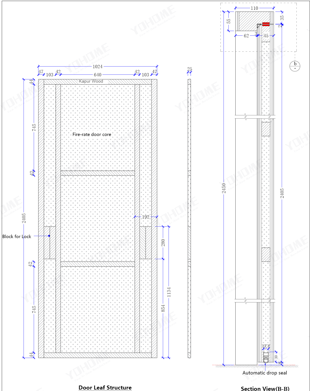
Interior Structure Drawing of UL 20mins single leaf wooden fire door and frame, model YH-01
