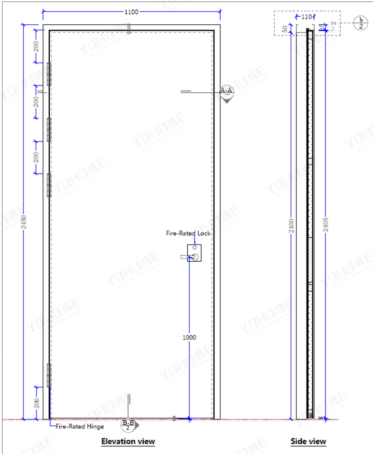
Drawing of UL 45mins single leaf wooden fire door and metal frame, Model YH-04
