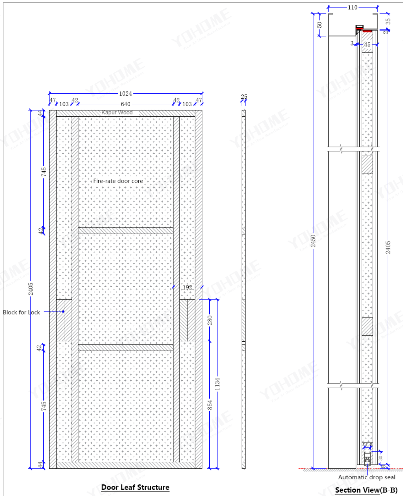
Interior Structure Drawing of UL 45mins single leaf wooden fire door and metal frame, model YH-04
