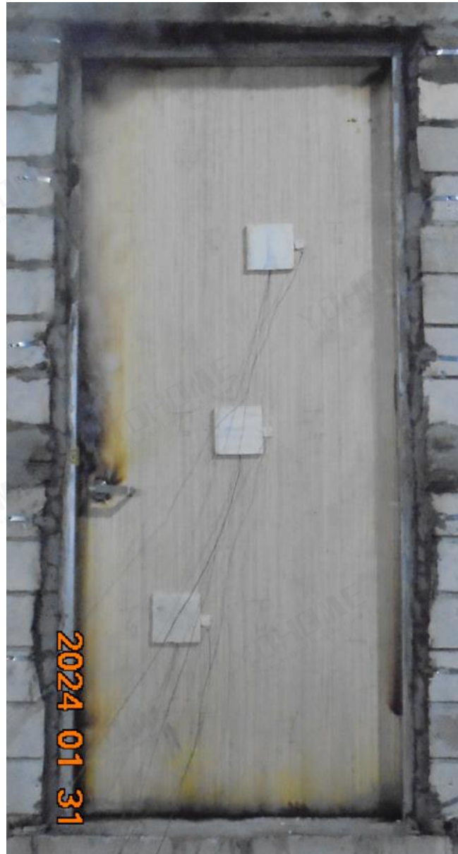
Photo No. 4 Unexposed Side after 30 Minutes
