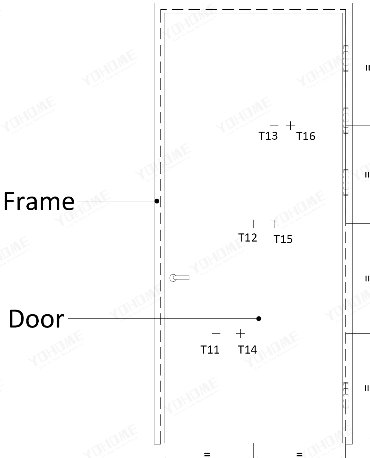
POSITION FOR MEASUREMENT OF UNEXPOSED TEMPERATURE
